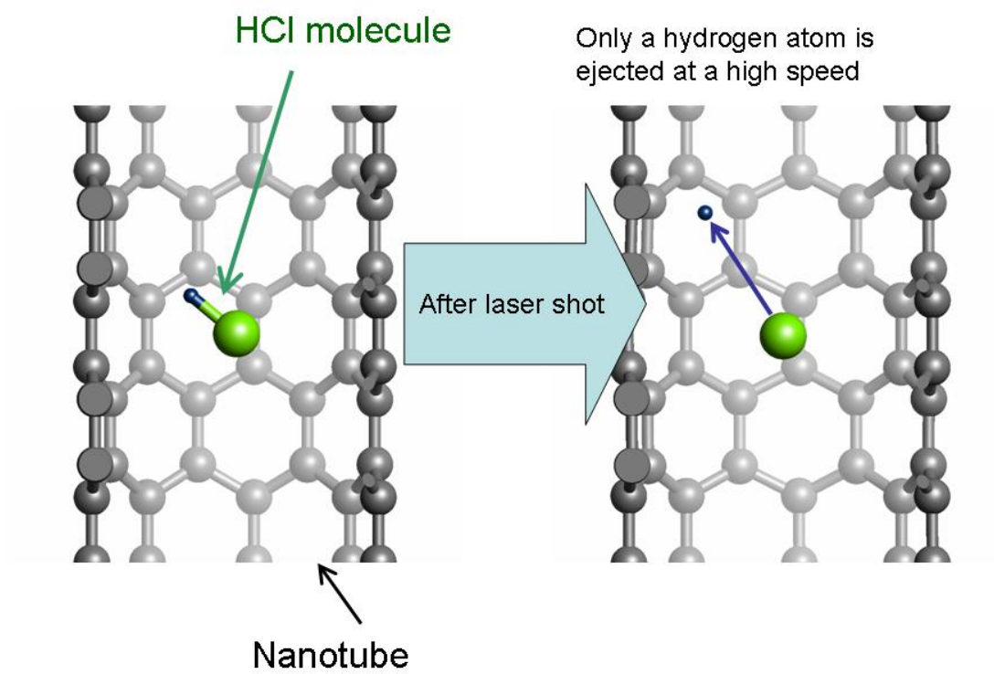
Figure: Dissociation of hydrogen chloride (HCl) molecule trapped inside a carbon nanotube due to the laser pulse irradiation.
